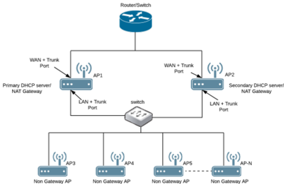
FIGURE 212 Hierarchical AP Topology
