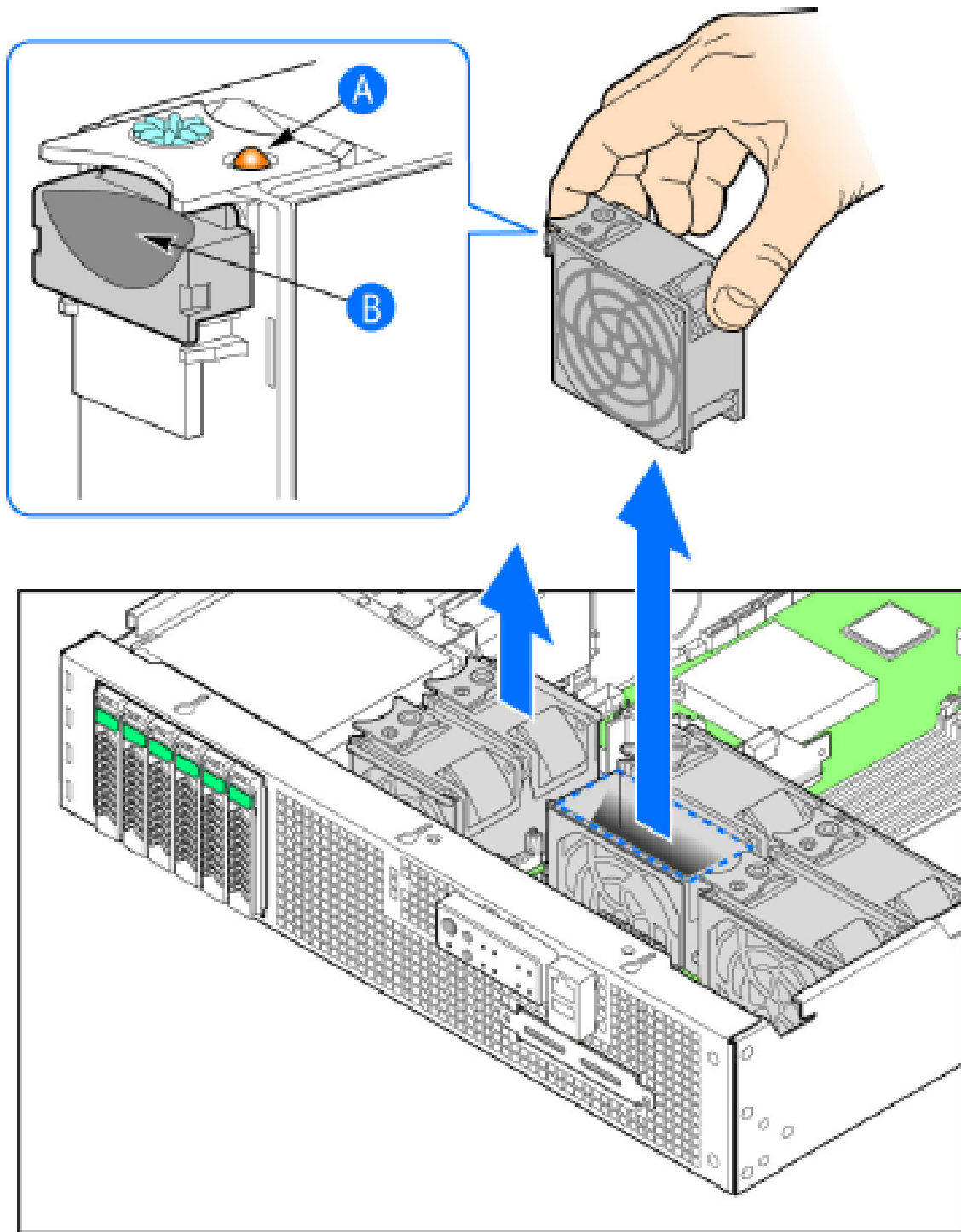
FIGURE 282 Replacing a system fan
