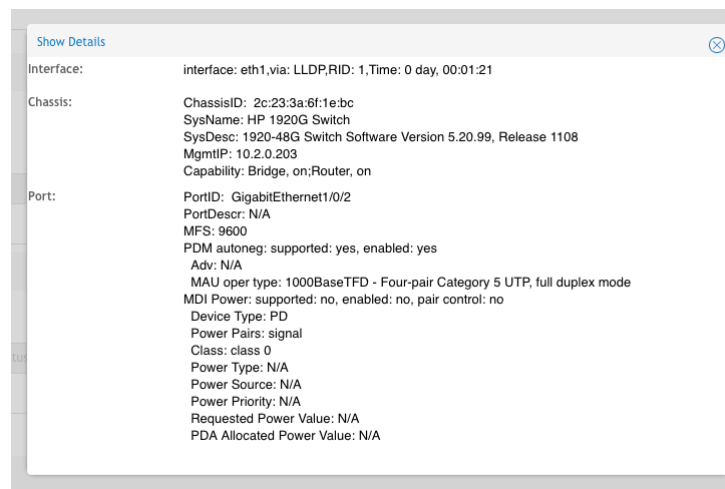
FIGURE 48 Additional LLDP AP Neighbor Details
