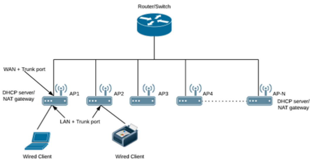
FIGURE 210 Single AP Topology
