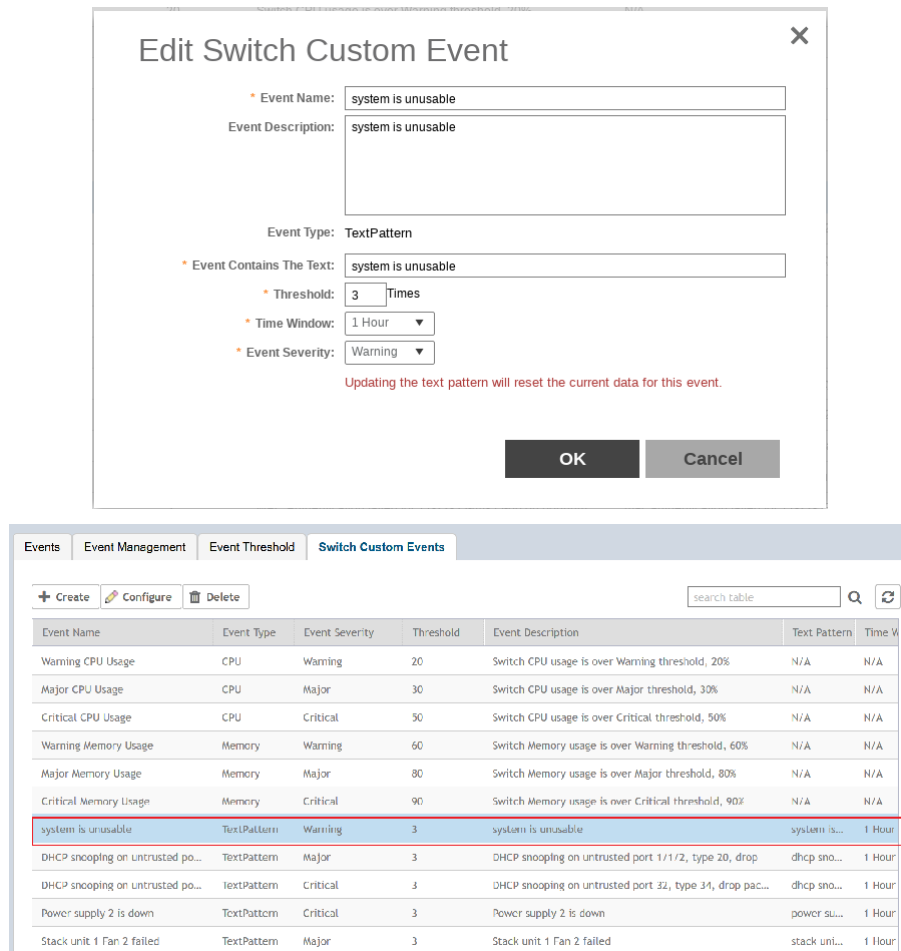
FIGURE 116 Troubleshooting switch issues through custom events
