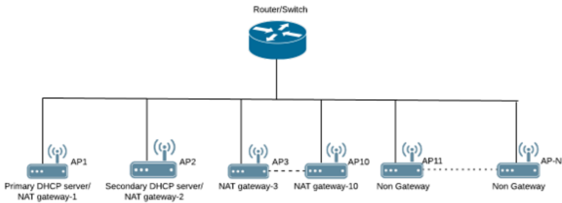
FIGURE 211 Multiple AP (Flat Network) Topology
