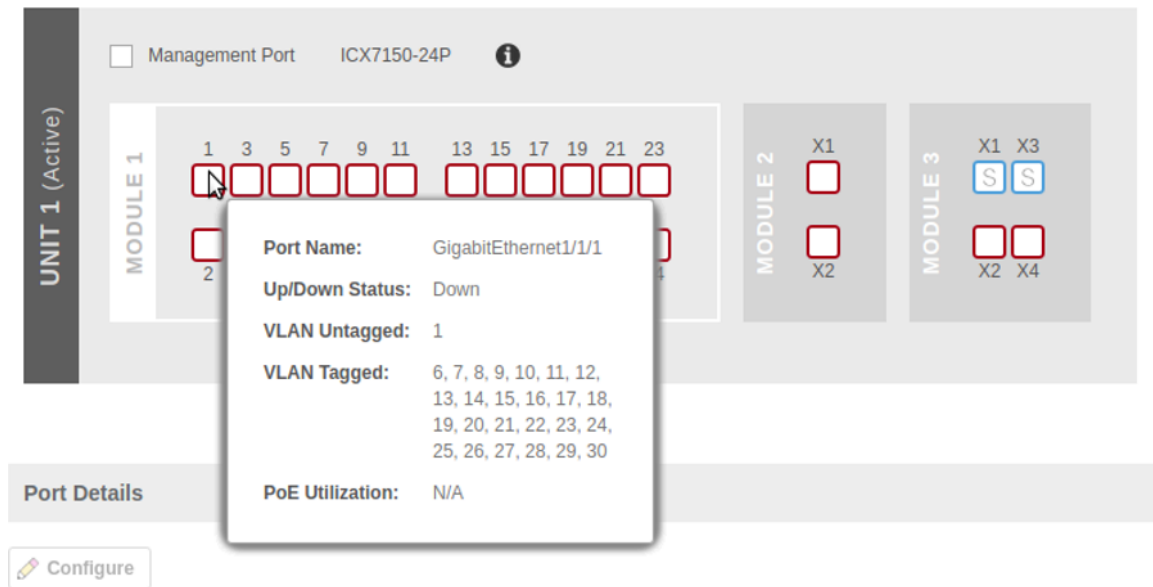
FIGURE 103 Front Panel View
