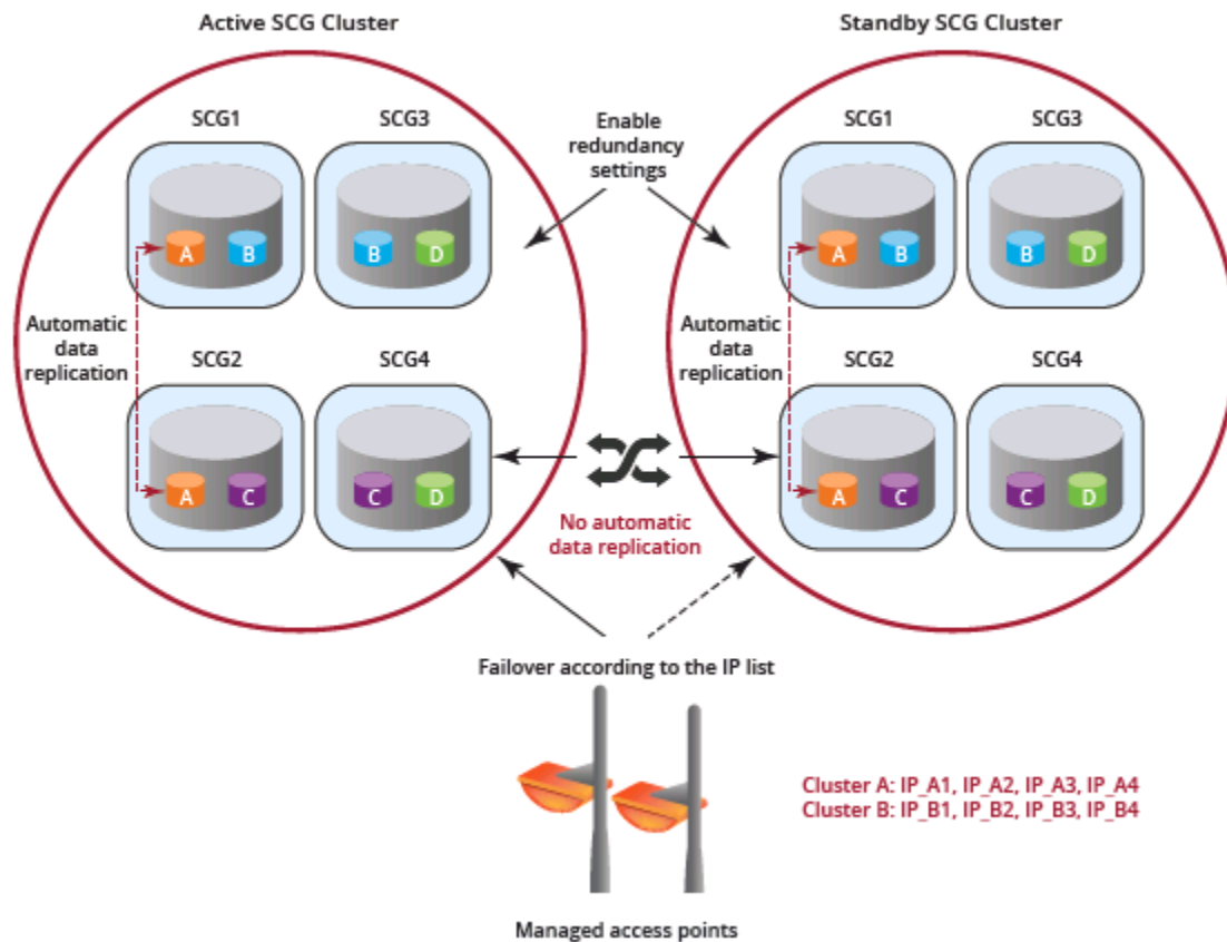
FIGURE 59 Cluster Redundancy for Active-Standby Mode
