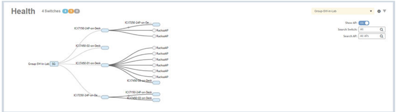
FIGURE 120 Showing Wired Devices Using Topology View Mode
